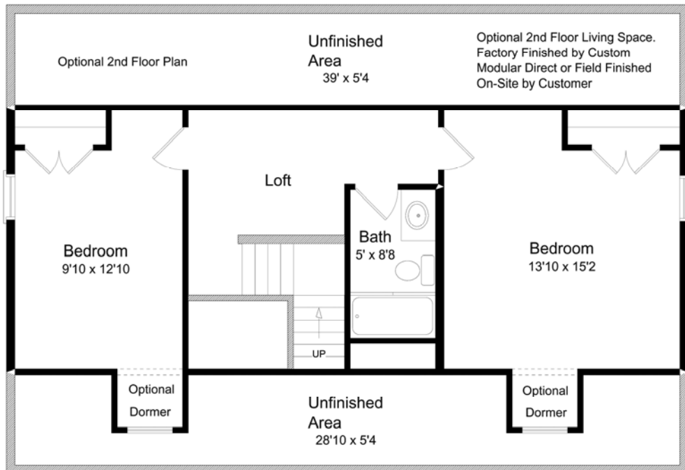
All Dimensions are Approximate
