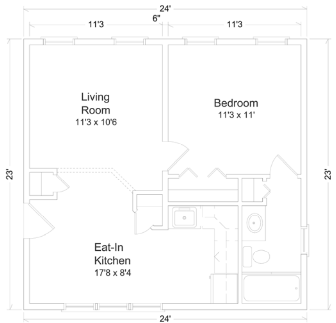
In-Law Suite 4 552 Sq. Ft.
