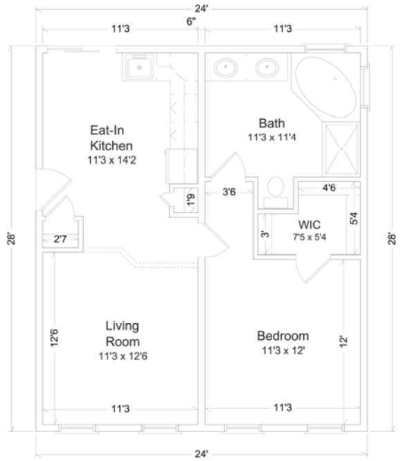
In-Law Suite 2 672 Sq. Ft.
