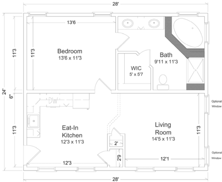
In-Law Suite 1 672 Sq. Ft.
