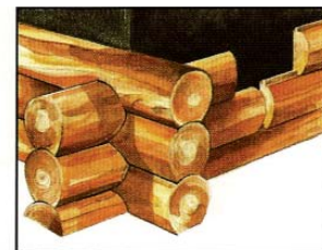
Swedish Cope profile; Dovetail also available
