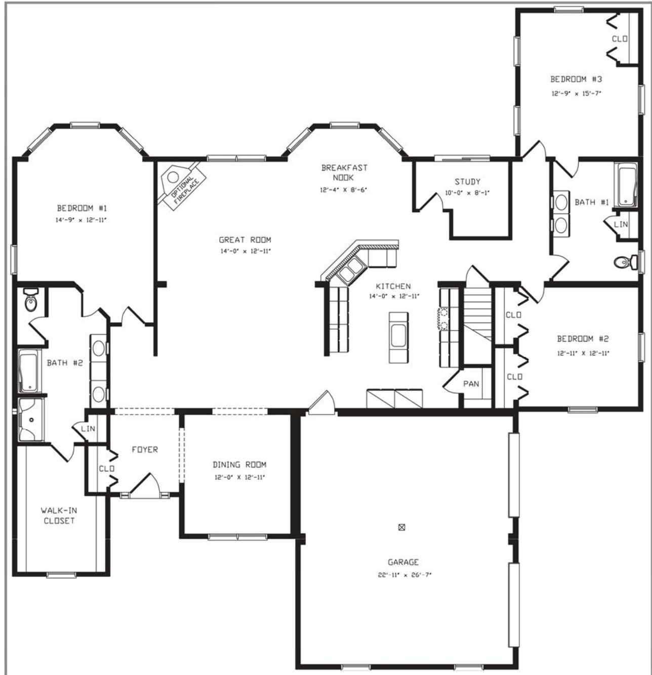
First Story
