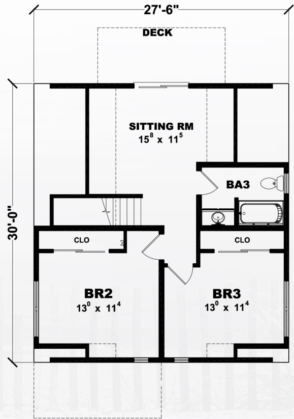
Proposed 2nd Floor
